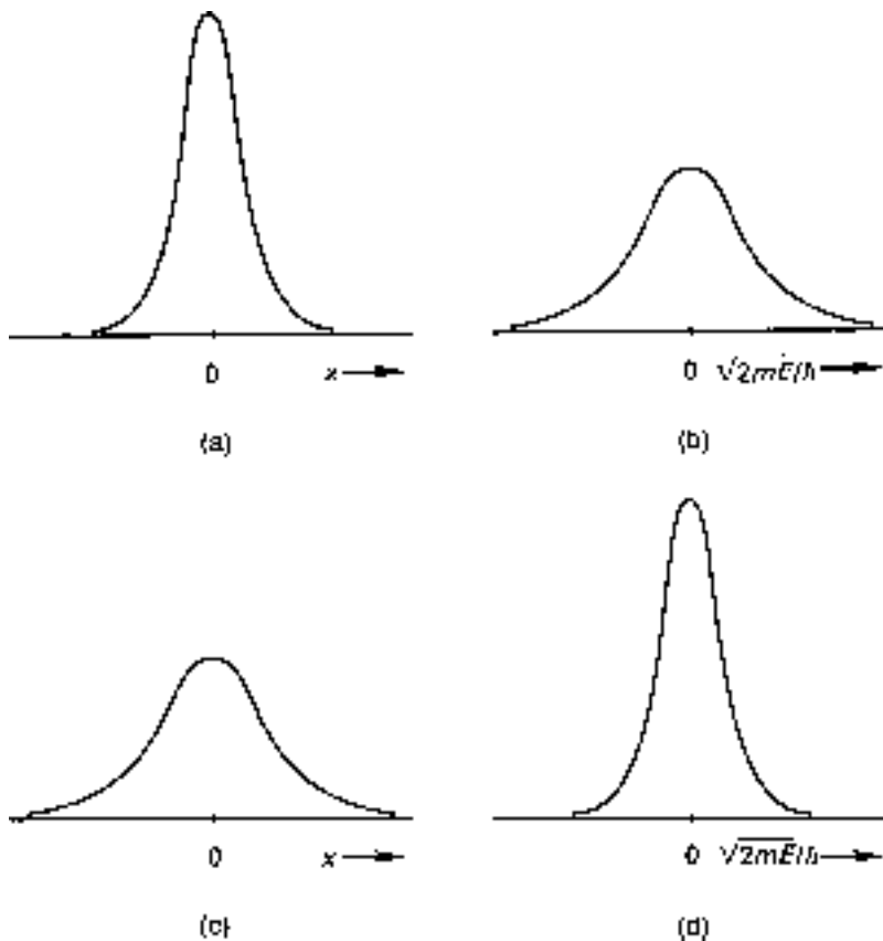
Figure 6-4 ► (a and c) Gaussian wave packets describing particles found to be at x=0 with differing degrees of certainty. (b and d) Values of c_k (where k = \sqrt{2mE}/\hbar ) for momentum eigenfunctions that combine to express the gaussian wave packets to their left. (a, b) corresponds to relatively certain position and relatively uncertain momentum, whereas (c, d) corresponds to the opposite situation.
