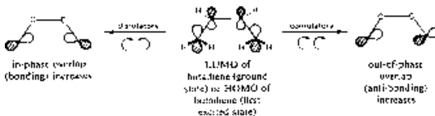
Figure 14-19 ► The HOMO of the first excited state of cis -1,3-butadiene as it undergoes closure by either mode.
