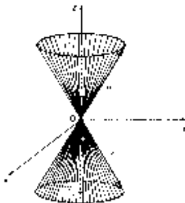
Figure 5-3 ► The angular momentum vectors for \alpha and \beta precess around the magnetic field axis z . The z components of these vectors are constant and have values of +\frac{1}{2} and -\frac{1}{2} a.u. respectively.
