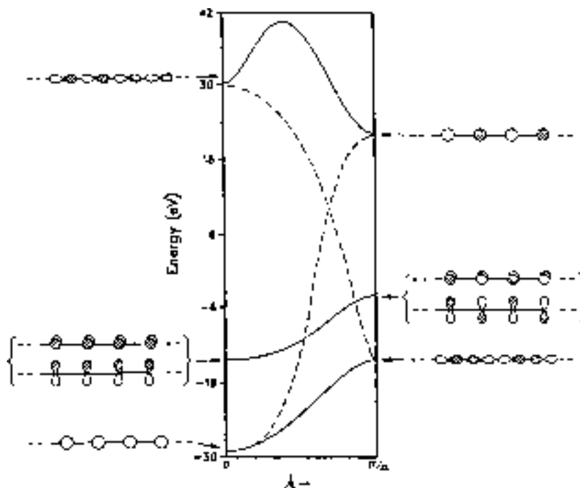
Figure 15-14 ► Band diagram for a linear chain of carbon atoms showing some COs and intended correlations. Positive and negative phases are indicated by shading or lack of shading. (From Hoffmann et al. [1].)
