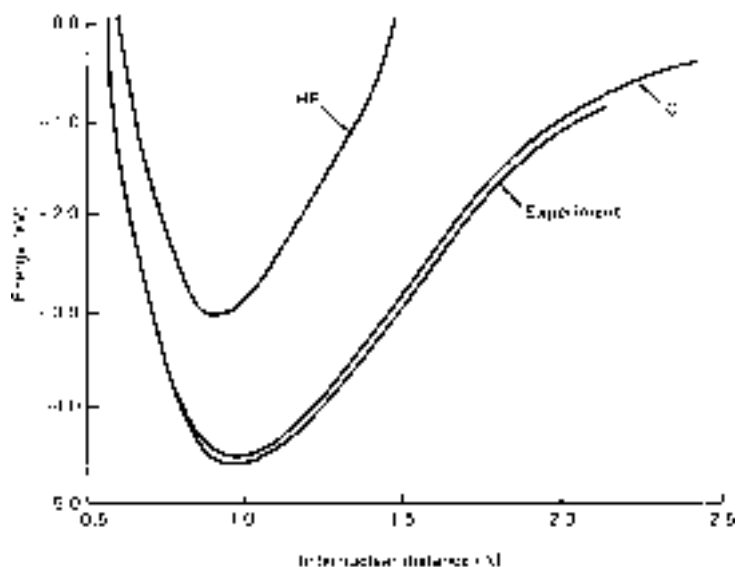
Figure 11-5 ► Theoretical and experimental energy curves for OH (from Stevens et al. [22].)
