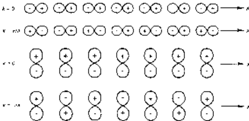
Figure 15-12 ► 2p_x and 2p_y basis sets at k=0, \pi/a .
