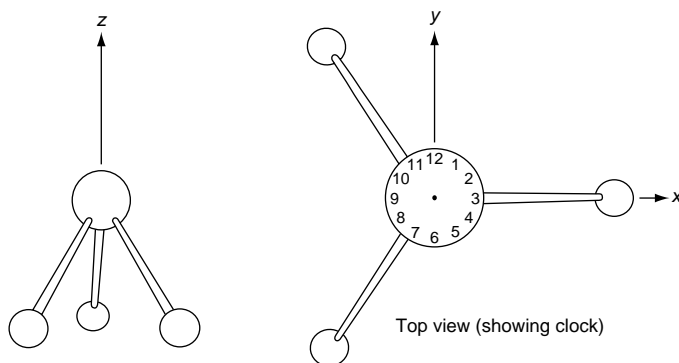
Figure 13-3 ► Orientation of a model of ammonia in Cartesian space.
