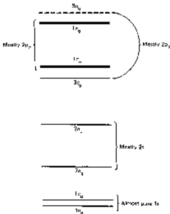
Figure 7-14 ► Schematic of MO energy level order for F_2 . The vertical axis is not an accurate energy scale. For instance, the 1\sigma levels are very much lower in energy relative to the other levels than is suggested by the drawing. (---) indicates that the orbital is unoccupied in the ground state.
