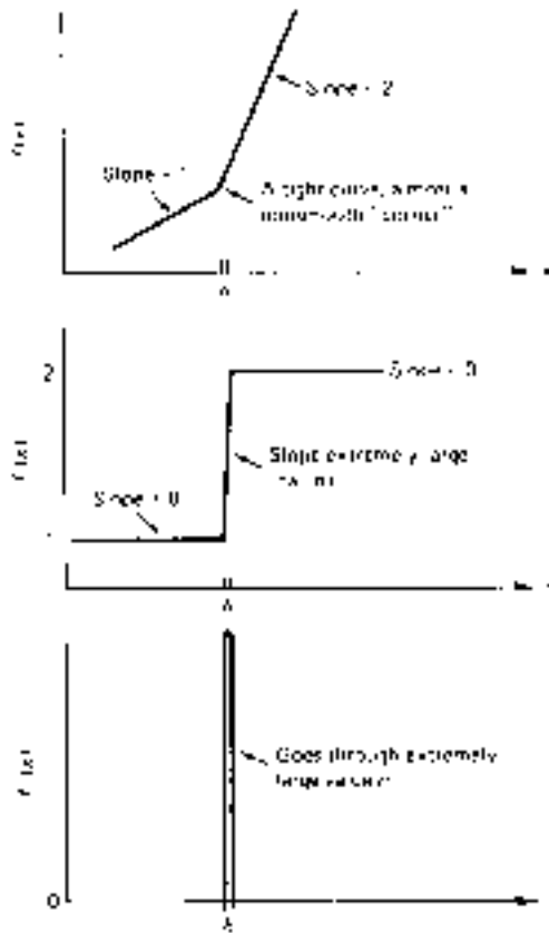
Figure 2-2 ▶ As the function f(x) approaches being nonsmooth, \delta approaches zero (the width of one point) and n approaches infinity.
