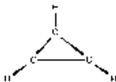
Figure 8-6 ► The cyclopropenyl system (all nuclei are coplanar).
