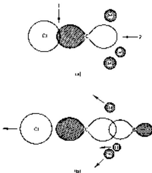
Figure 14-28 ► (a) The LUMO of \text{CH}_3\text{Cl} . (b) Positive overlap between HOMO of base B and LUMO of \text{CH}_3\text{Cl} increases antibonding between C and Cl and also repels H atoms from their original positions.
