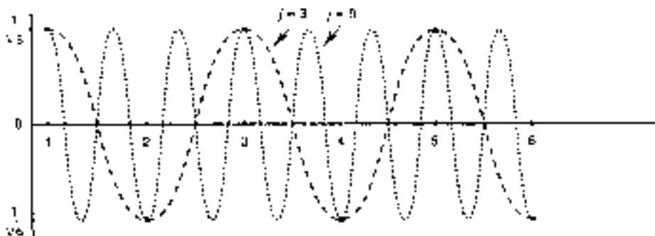
Figure 15-6 ► Coefficient waves for j=3 (dashed curve) and j=9 (dotted curve). Both curves intercept the same coefficient values ( \pm 1/\sqrt{6} ) at the positions related to carbon atoms 1–6, so the curves produce the same MO.
